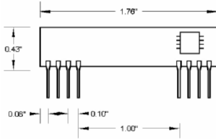
Mechanical Drawing
