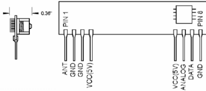
Pinout Diagram
